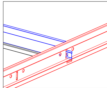
Detail B : Long Cross Carrier 1200 mm to Short Cross Carrier 600 mm Connection Detail
