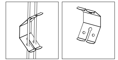
Detail D : Double Spring Clip (Spring Steel) 3D View
