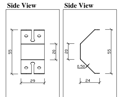
Anchor (Steel)
