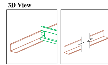
Detail C : L Perimeter Trim (Pre-Paint Steel) 3D View
