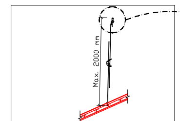
Detail F : Hanger Wire (Ø 4mm - Galvanized Steel)
