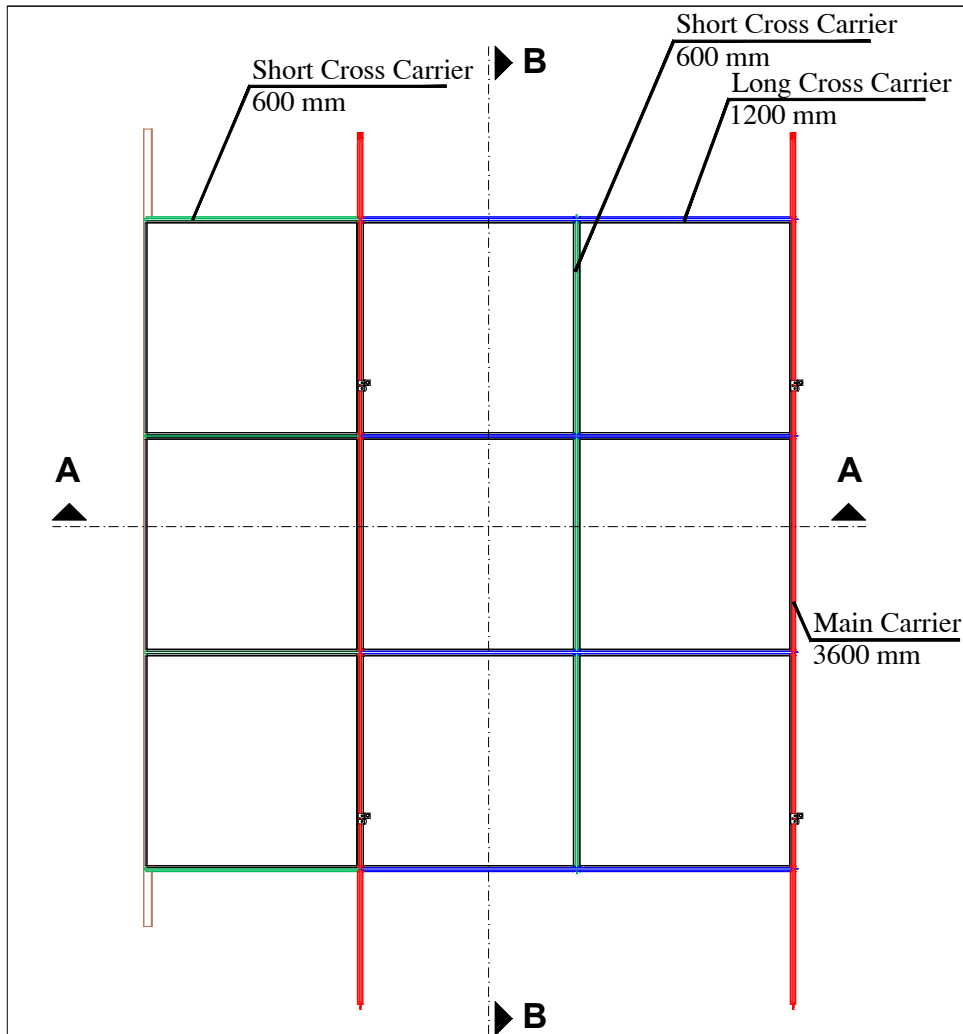
System Plan
