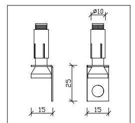
Anchor (Steel)
